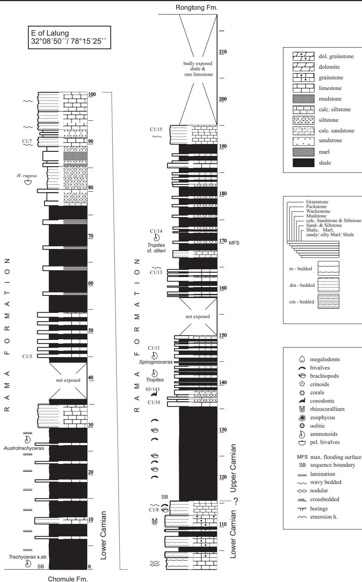
Figure 8: Stratigraphic log of the Rama Formation (type section), E of Lalung.
