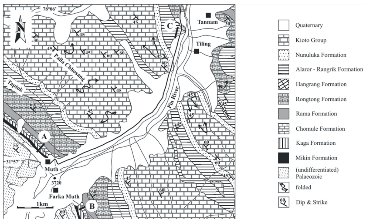
Figure 1: Geology of Muth (after Fuchs, 1982) with position of sections E/M 03 (A), Muth 3 near Farka Muth (B) and opposite Tiling (C).
